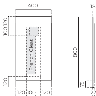
French Cleat Fixing System
