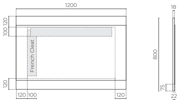
French Cleat Fixing System
